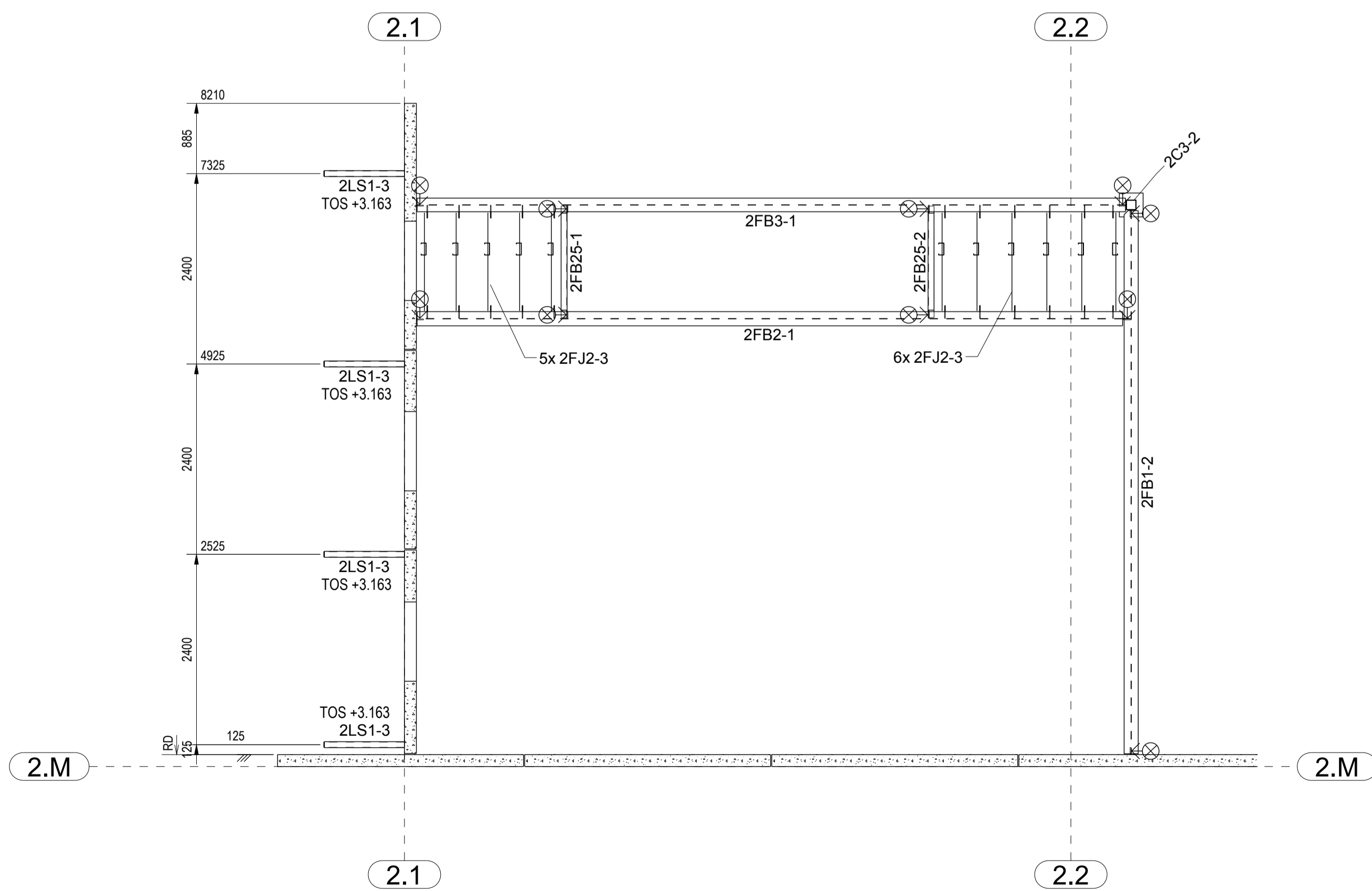
MAZZANINE UNIT 10 MARKING PLAN
