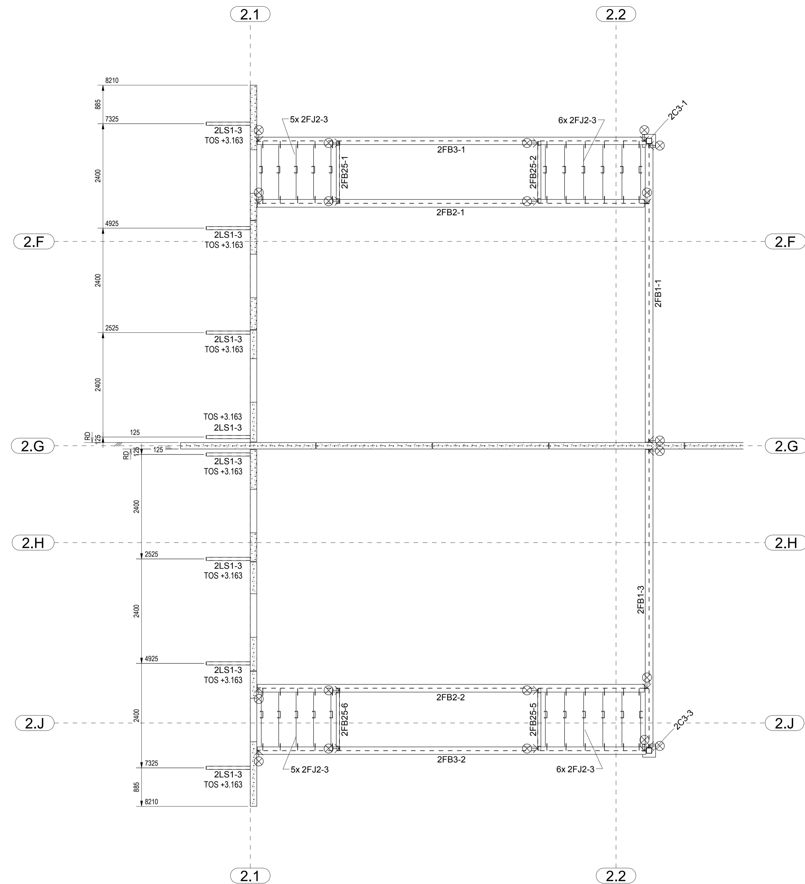
MAZZANINE UNITS 16 & 17 MARKING PLAN
